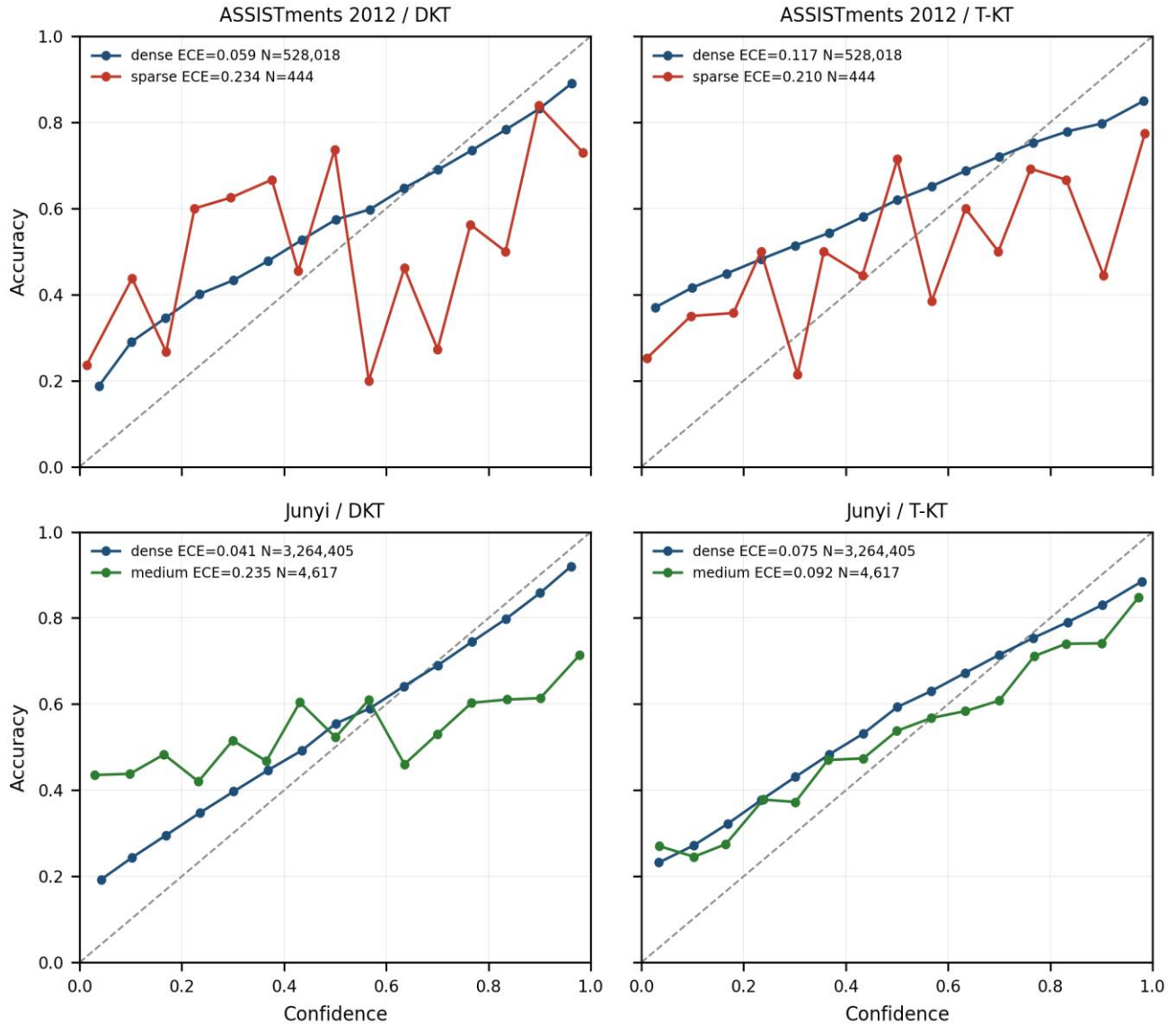
Fig. 3. Reliability diagrams (15 equal-width bins; seed 42 only) are visual diagnostics. Tables 5 and 6 report four-partition means. Rows: ASSISTments 2012 and Junyi Academy. Columns: DKT and T-KT. ASSISTments panels show dense vs sparse; Junyi panels show dense vs medium (learner-based sparse is empty). Not a classroom trial.
